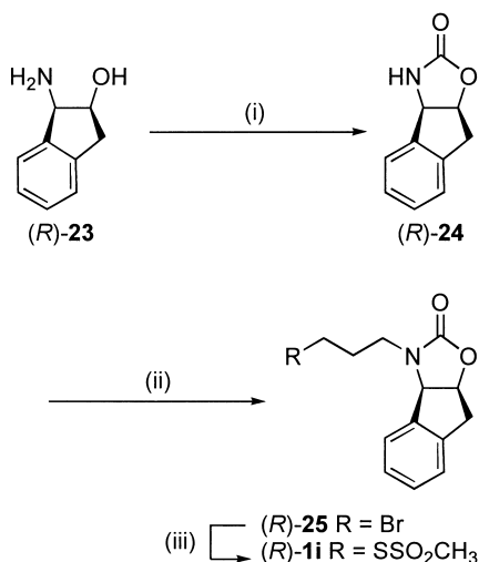
Scheme 4. Reagents: (i) Triphosgene, CH 2 Cl 2 , Et 3 N, 100%; (ii) KOH, DMSO, Br(CH 2 ) 3 Br; (iii) NaSSO 2 CH 3 , DMF.
