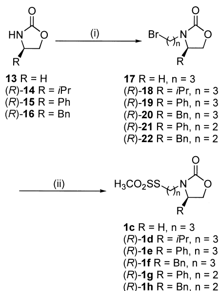
Scheme 3. Reagents: (i) KOH, DMSO, Br(CH 2 ) n Br; (ii) NaSSO 2 CH 3 , DMF.
