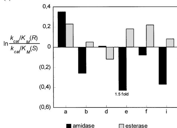
Figure 1. Comparison of specificity constants for N62C, S166C and L217C CMMs.
