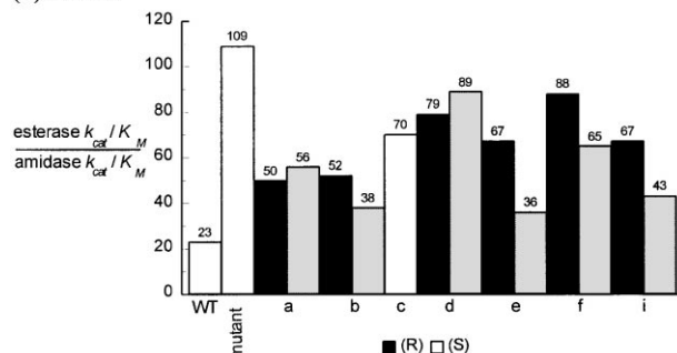
Figure 2. Changes in esterase to amidase activity ratios for S166C and L217C CMMs.
